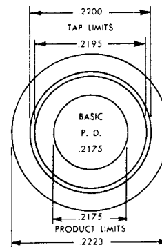
Class 2B Limit GH-5 Tap
