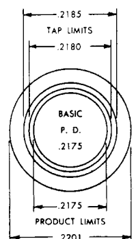
Class 3 Limit GH-2 Tap
